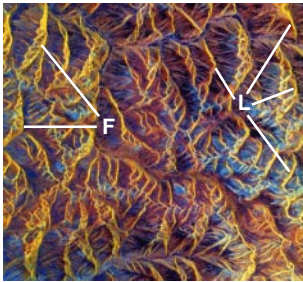
A color display of SIR-C radar bands covering a rugged mountainous area in southeast Tibet. The look direction is toward the left side of the image. The labels indicate several of the many examples of foreshortening (F) and layover (L) of slopes facing the sensor.
